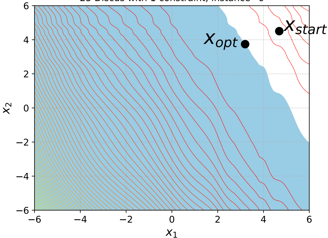
25 Discus with 1 constraint, instance=6
