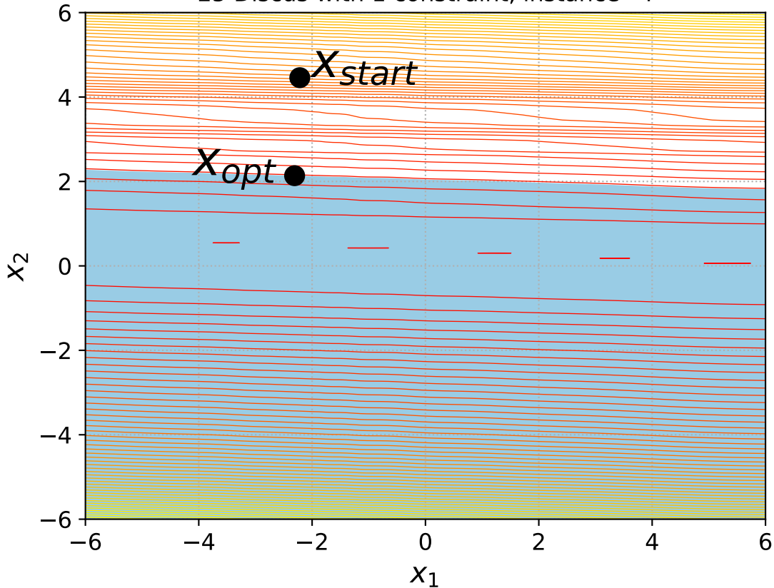
25 Discus with 1 constraint, instance=4
