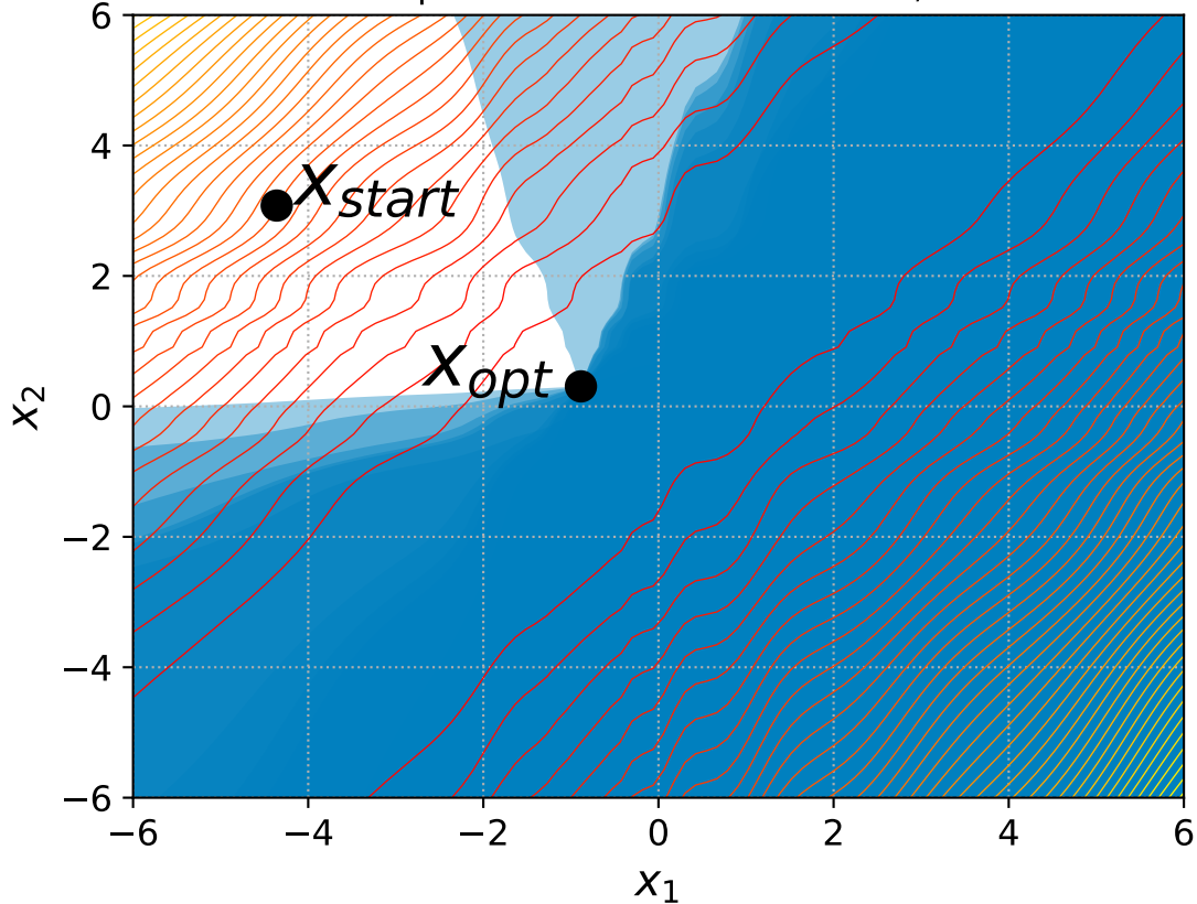
24 Rotated Ellipsoid with 6+3n constraints, instance=15
