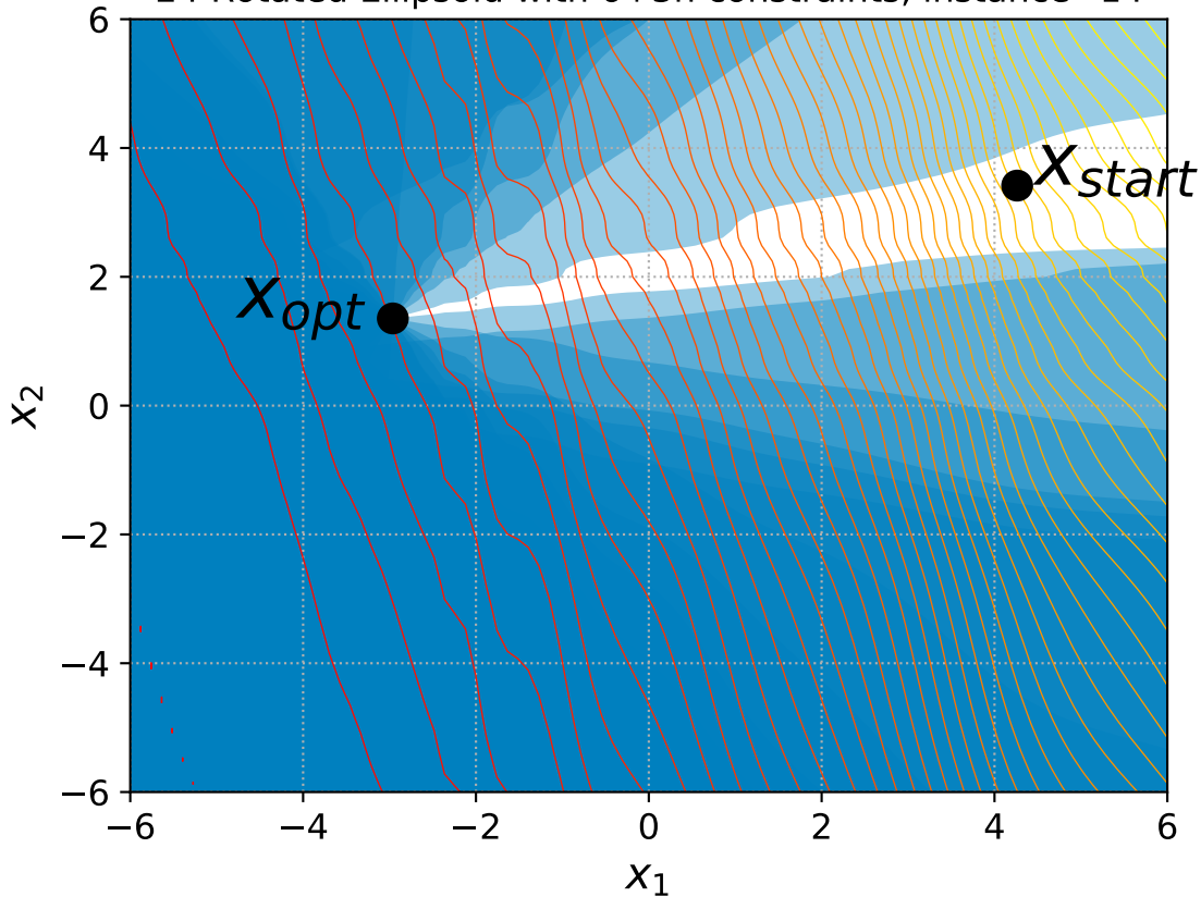
24 Rotated Ellipsoid with 6+3n constraints, instance=14
