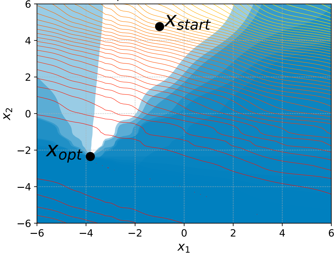
24 Rotated Ellipsoid with 6+3n constraints, instance=11
