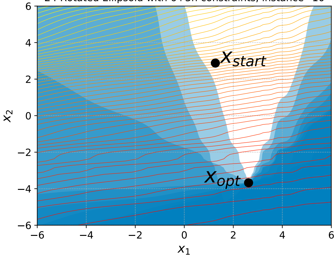
24 Rotated Ellipsoid with 6+3n constraints, instance=10
