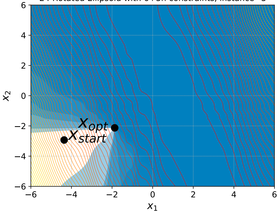
24 Rotated Ellipsoid with 6+3n constraints, instance=3
