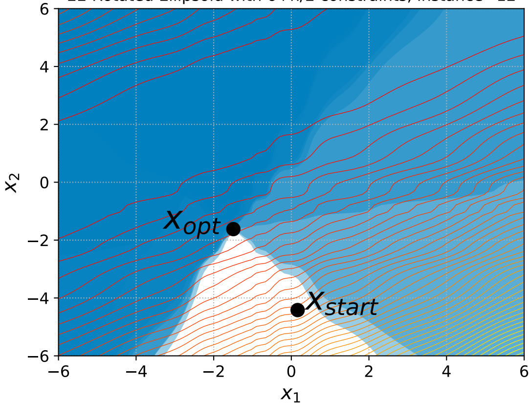
22 Rotated Ellipsoid with 6+n/2 constraints, instance=12
