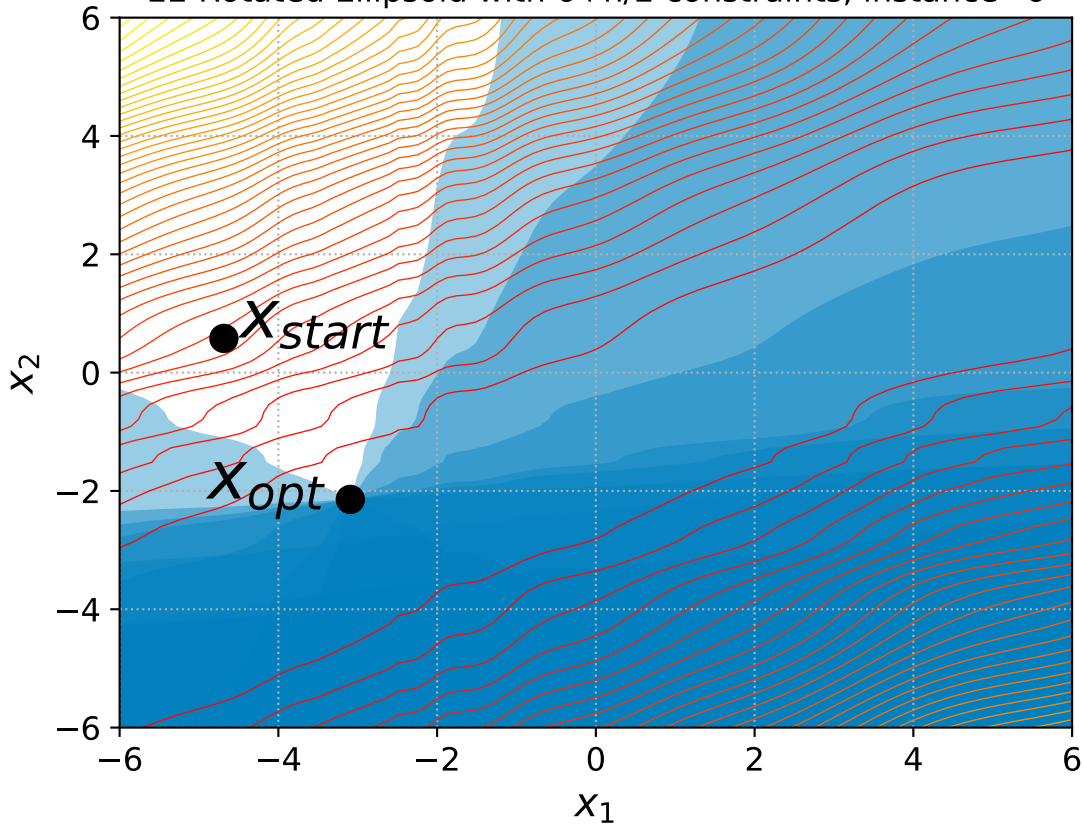
22 Rotated Ellipsoid with 6+n/2 constraints, instance=6
