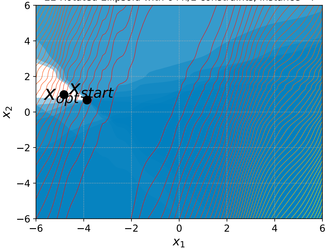
22 Rotated Ellipsoid with 6+n/2 constraints, instance=4
