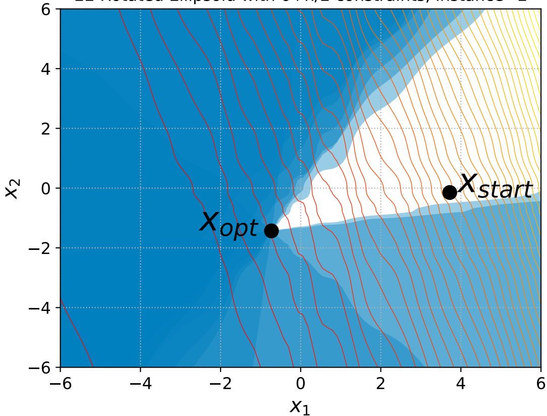
22 Rotated Ellipsoid with 6+n/2 constraints, instance=2
