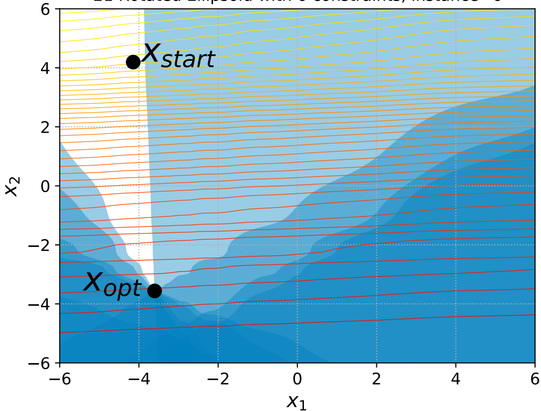
21 Rotated Ellipsoid with 6 constraints, instance=6
