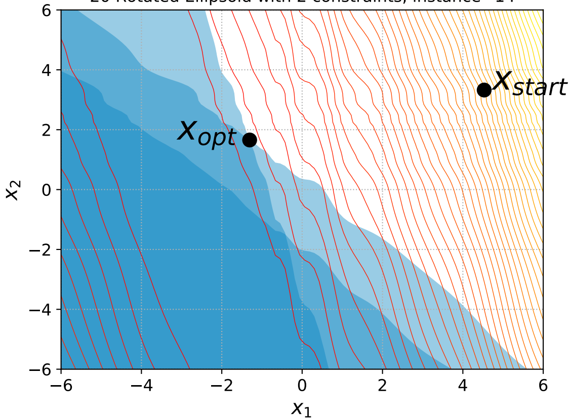
20 Rotated Ellipsoid with 2 constraints, instance=14
