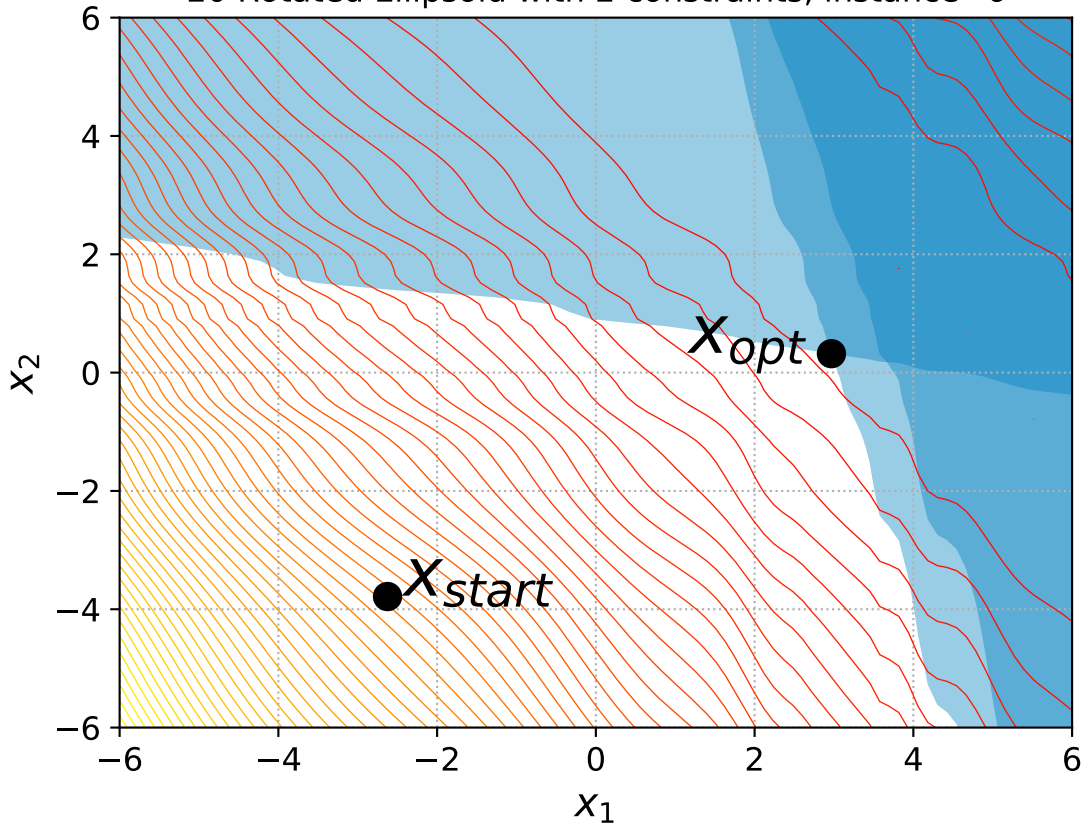
20 Rotated Ellipsoid with 2 constraints, instance=6
