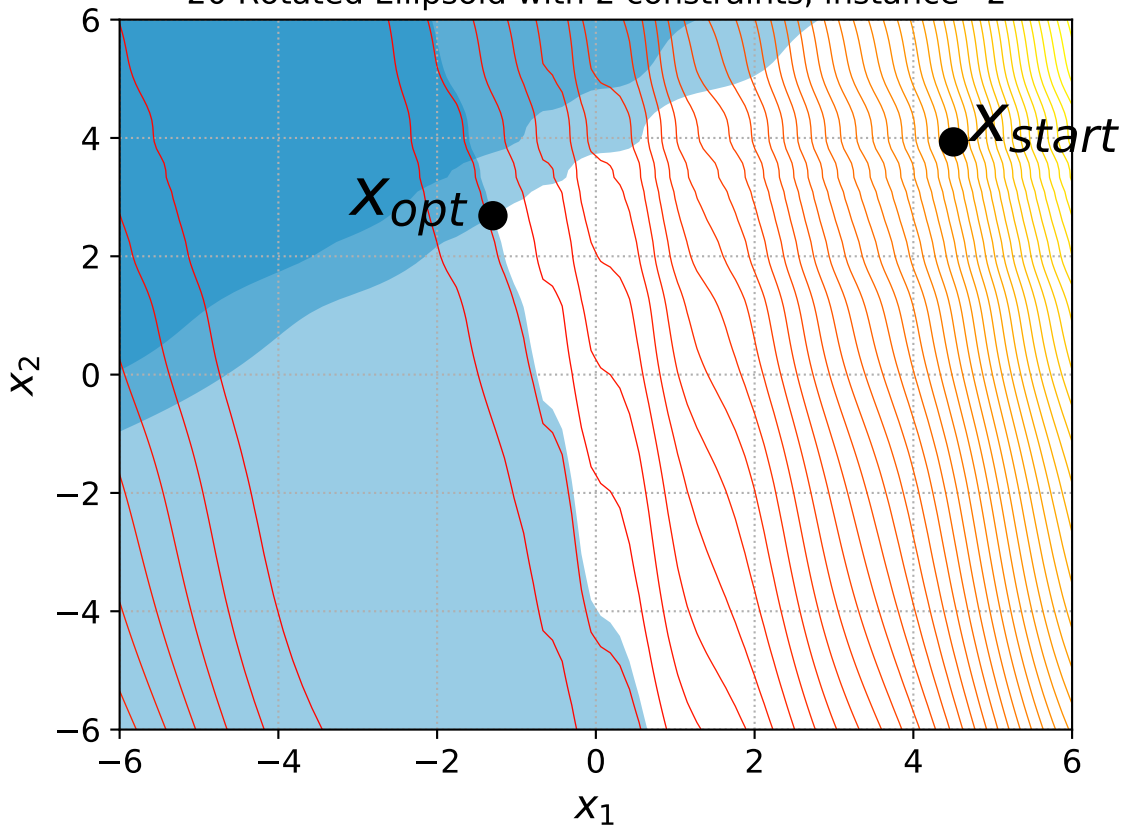
20 Rotated Ellipsoid with 2 constraints, instance=2
