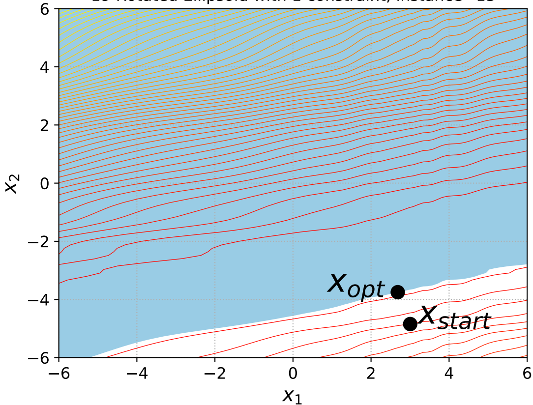
19 Rotated Ellipsoid with 1 constraint, instance=13
