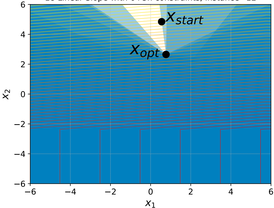
18 Linear Slope with 6+3n constraints, instance=12
