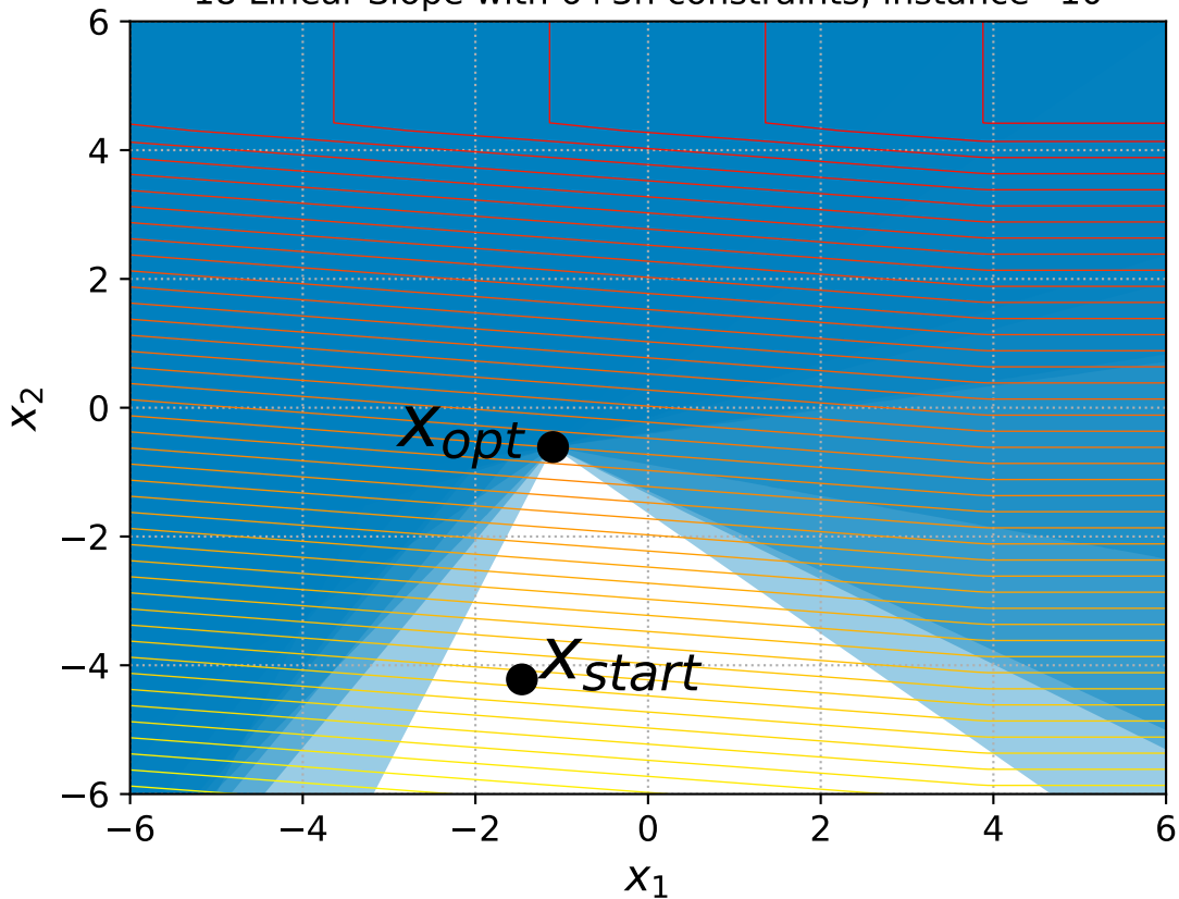
18 Linear Slope with 6+3n constraints, instance=10
