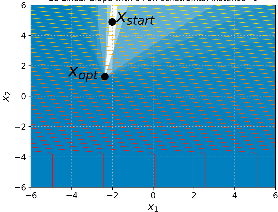
18 Linear Slope with 6+3n constraints, instance=9
