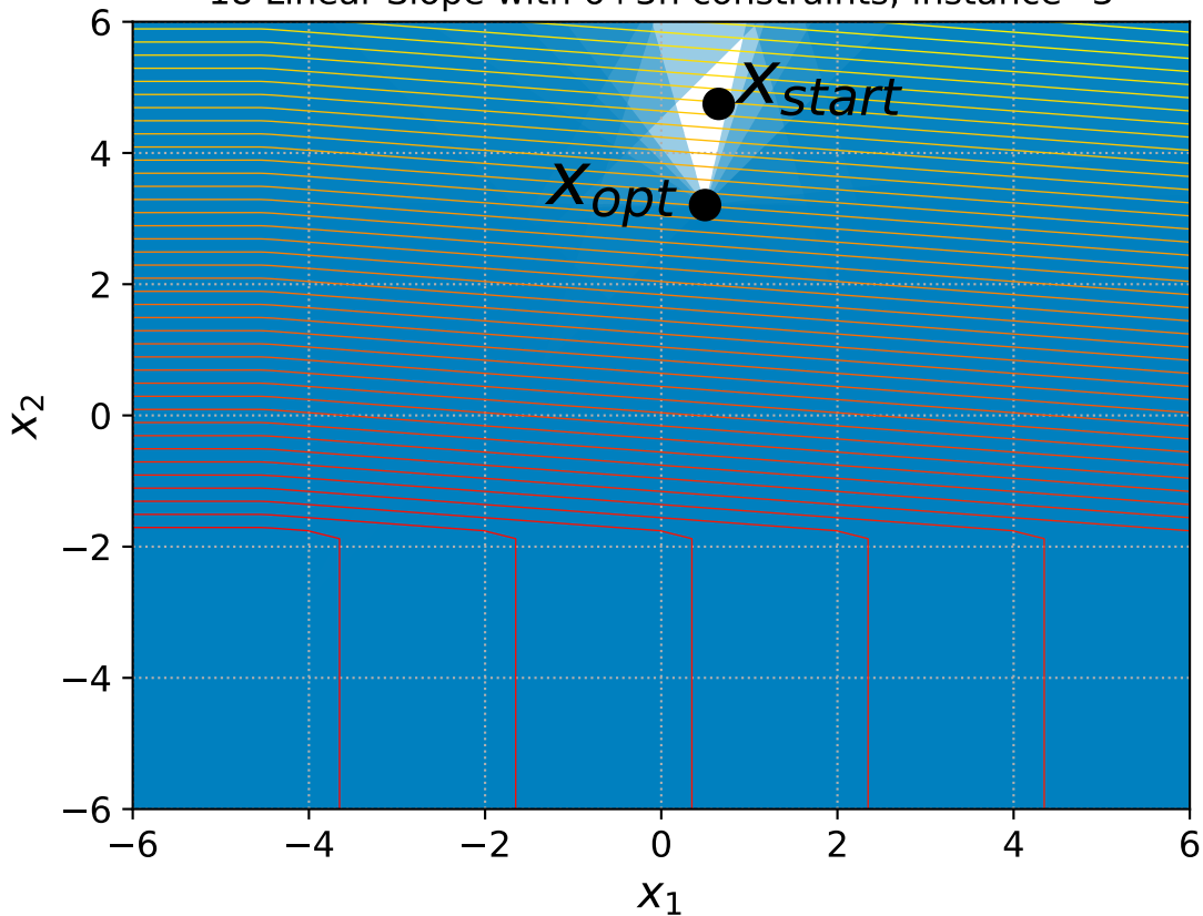
18 Linear Slope with 6+3n constraints, instance=3
