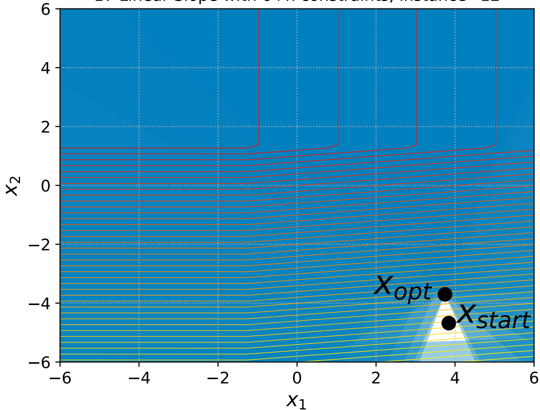
17 Linear Slope with 6+n constraints, instance=12
