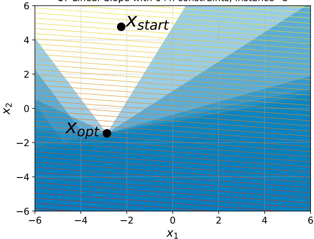
17 Linear Slope with 6+n constraints, instance=8
