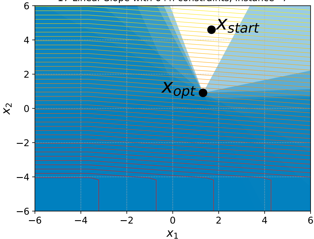
17 Linear Slope with 6+n constraints, instance=7
