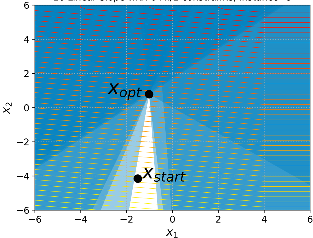
16 Linear Slope with 6+n/2 constraints, instance=9
