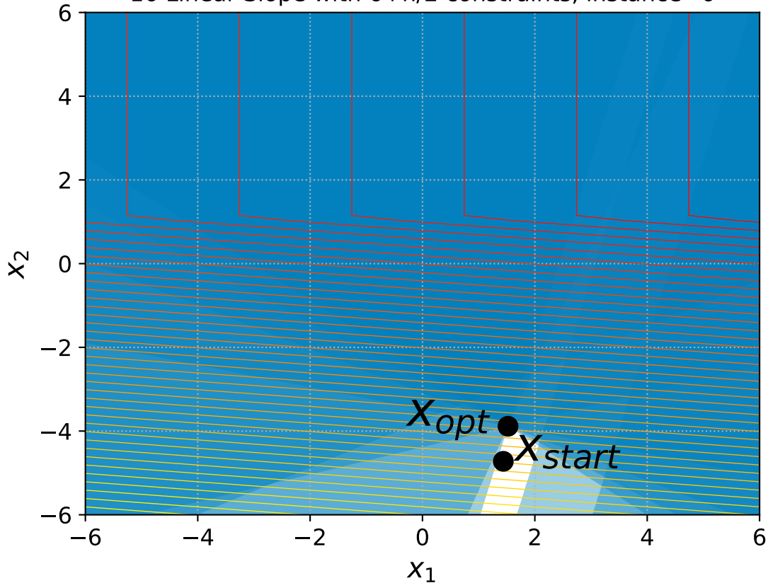
16 Linear Slope with 6+n/2 constraints, instance=6
