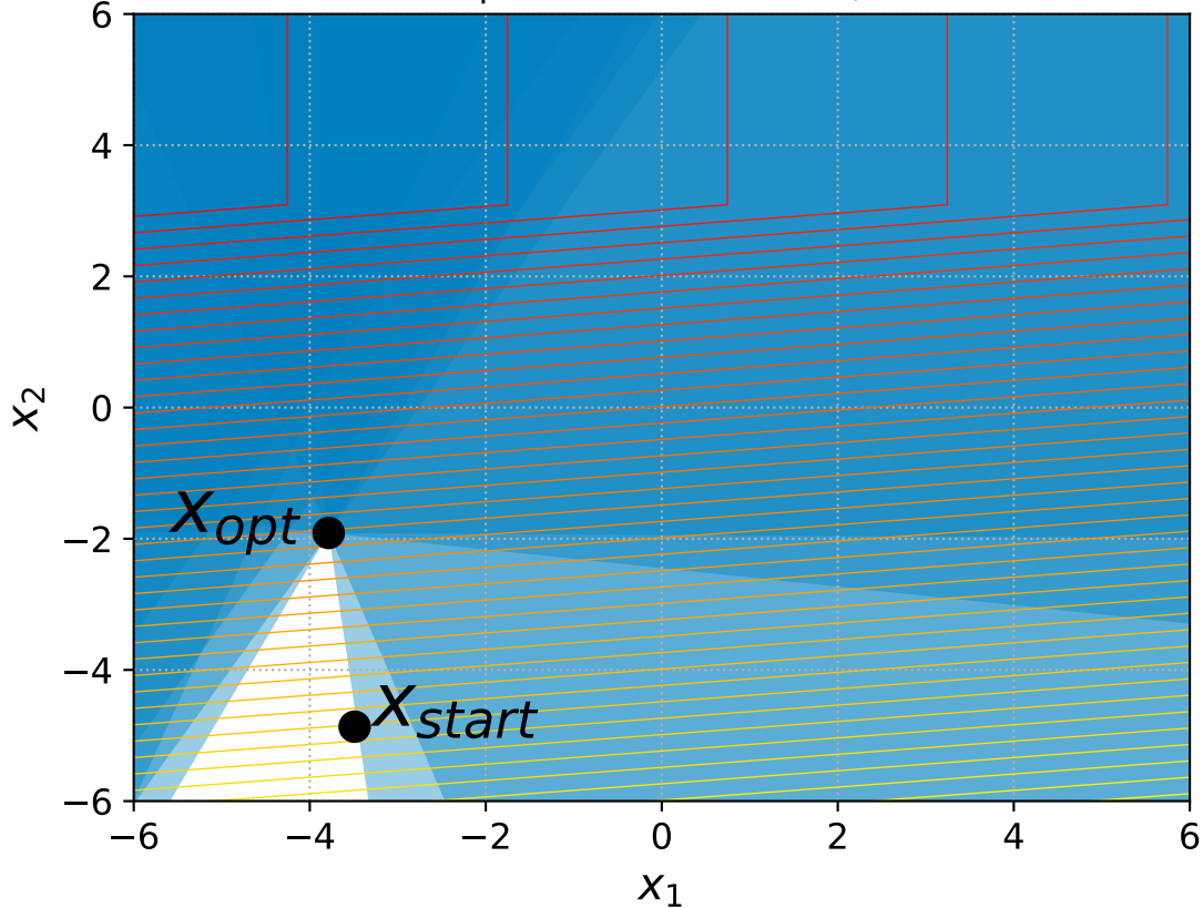
15 Linear Slope with 6 constraints, instance=4
