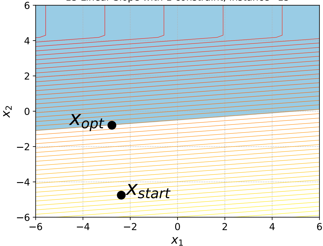
13 Linear Slope with 1 constraint, instance=15
