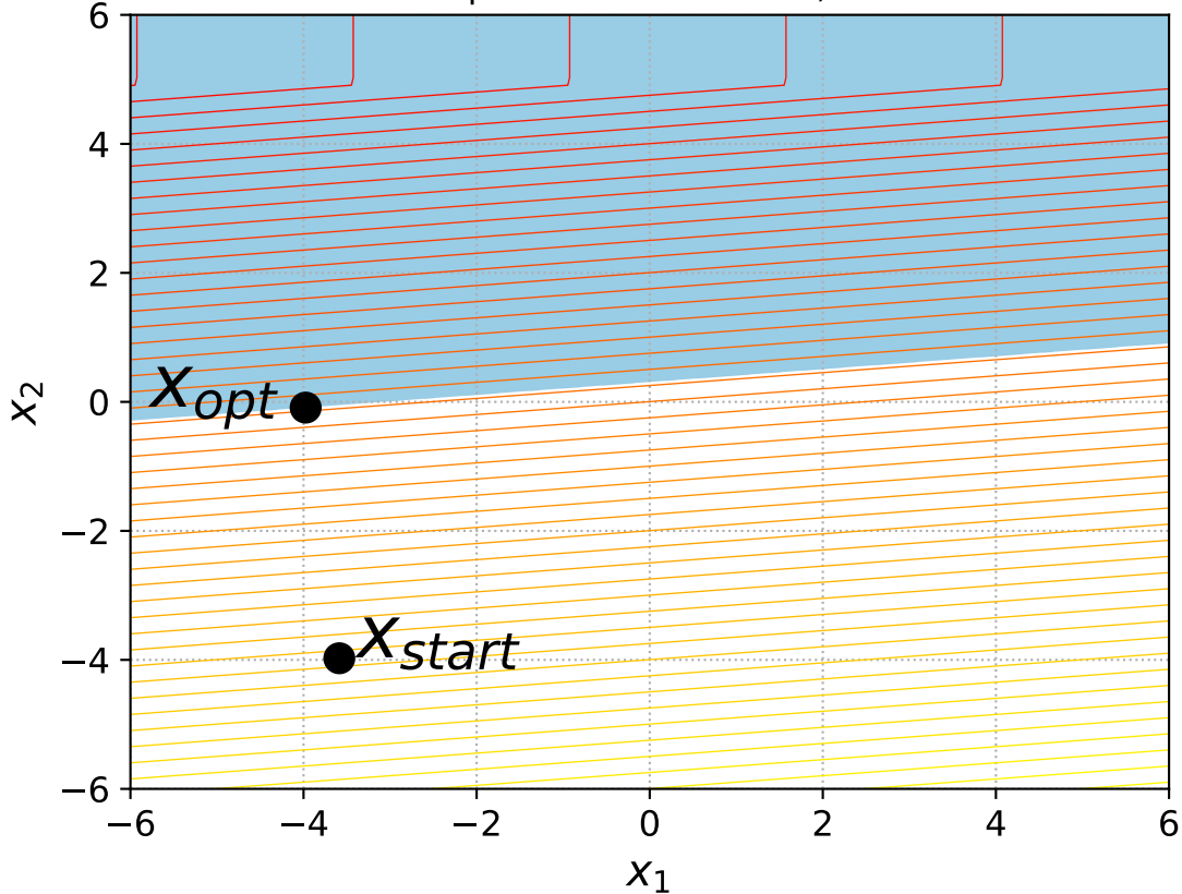
13 Linear Slope with 1 constraint, instance=11
