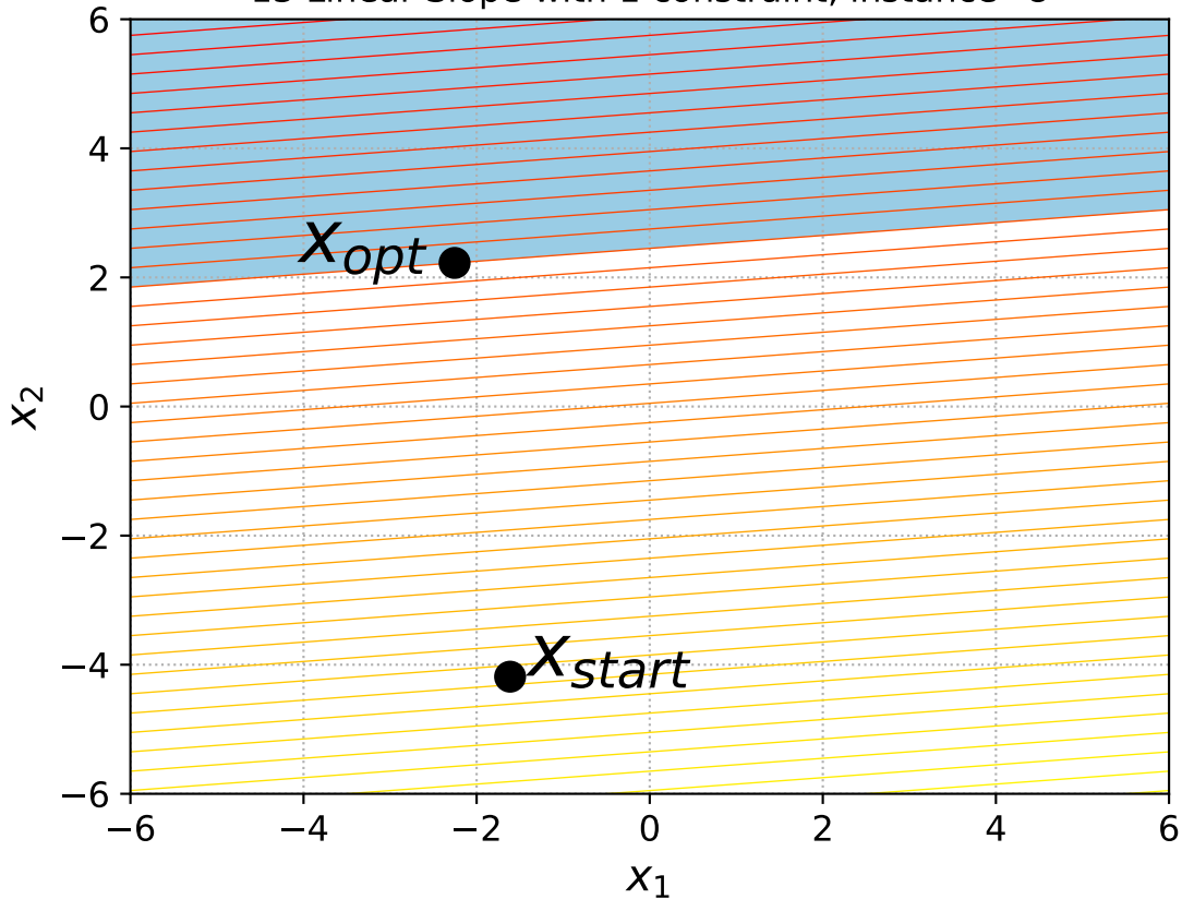
13 Linear Slope with 1 constraint, instance=8
