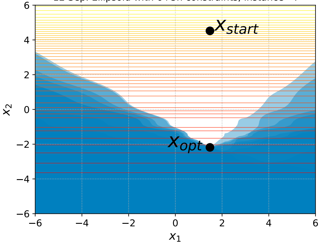
12 Sep. Ellipsoid with 6+3n constraints, instance=4
