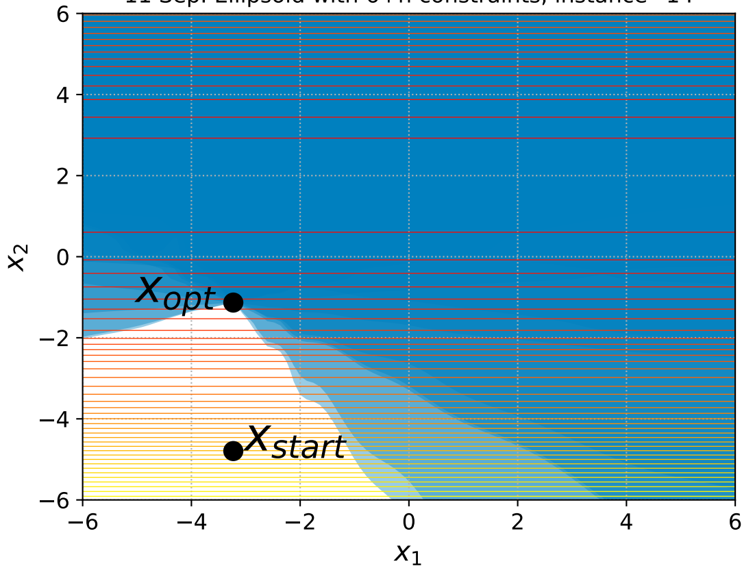
11 Sep. Ellipsoid with 6+n constraints, instance=14
