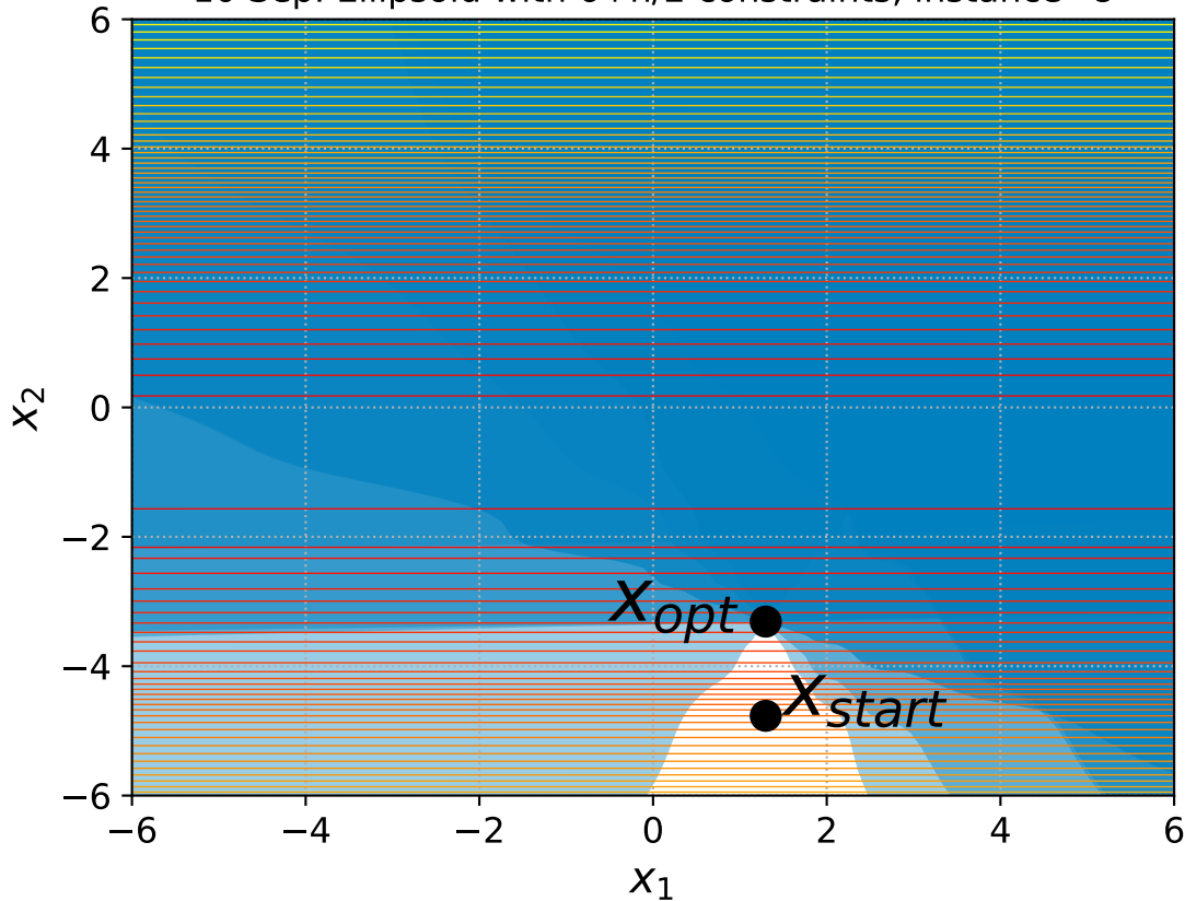
10 Sep. Ellipsoid with 6+n/2 constraints, instance=8
