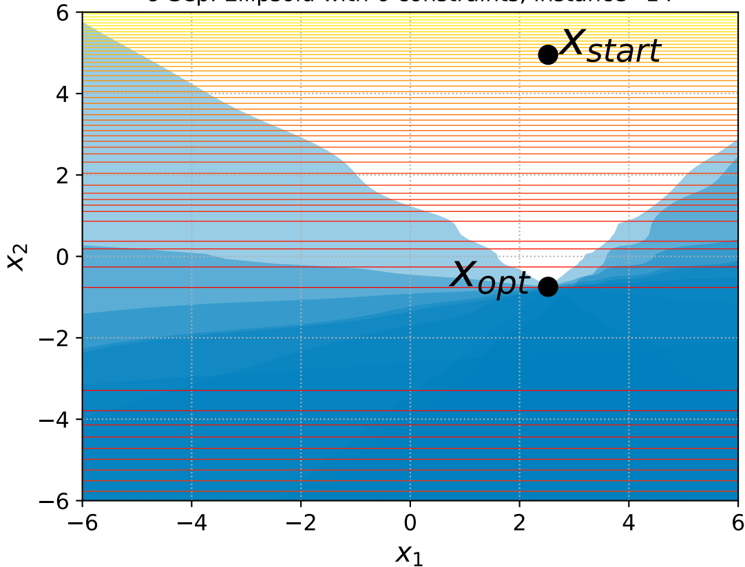
9 Sep. Ellipsoid with 6 constraints, instance=14
