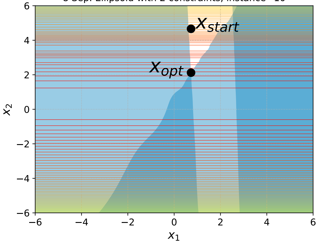
8 Sep. Ellipsoid with 2 constraints, instance=10
