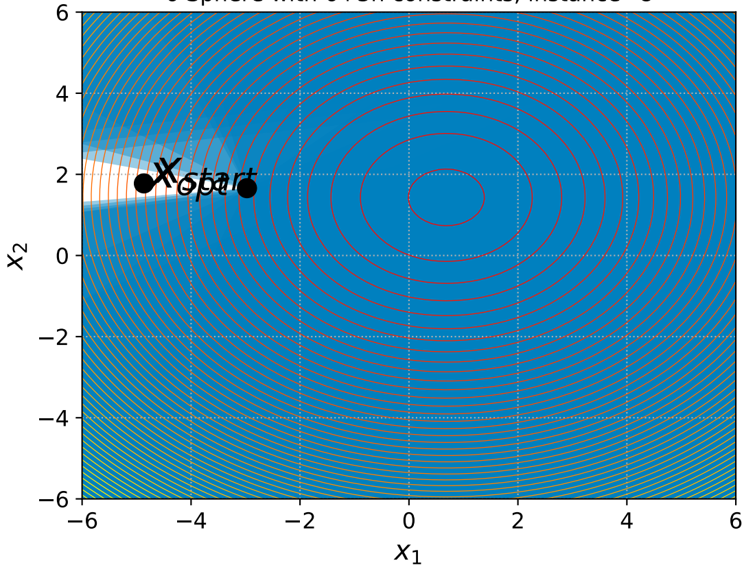
6 Sphere with 6+3n constraints, instance=8
