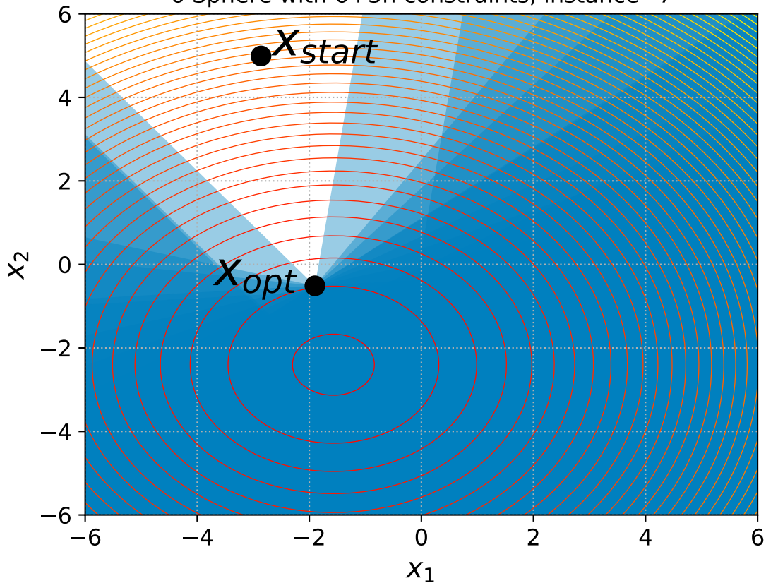
6 Sphere with 6+3n constraints, instance=7
