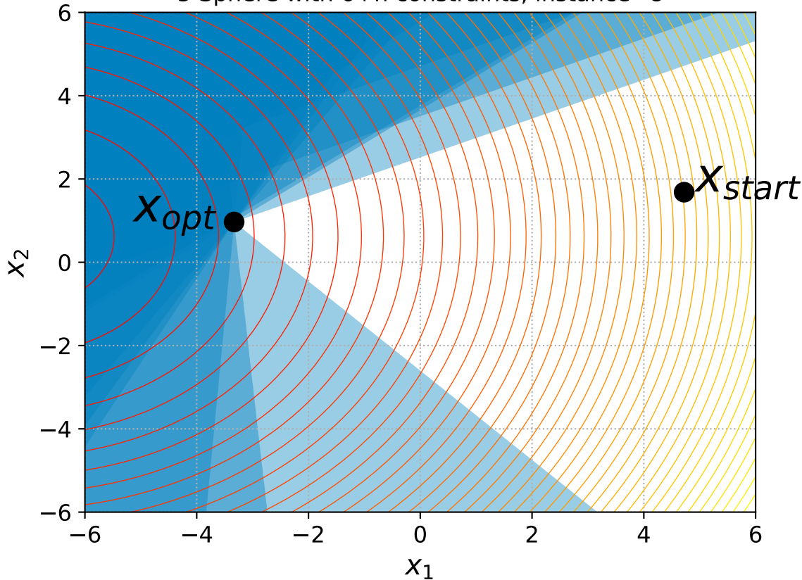
5 Sphere with 6+n constraints, instance=8
