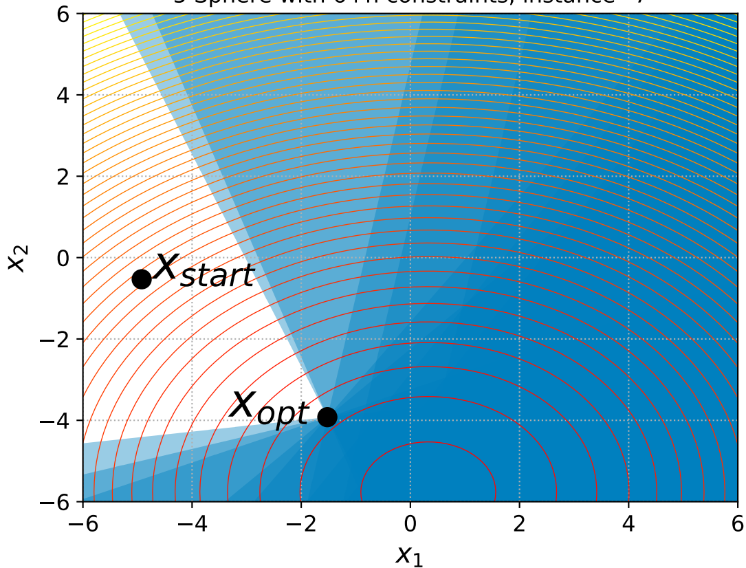
5 Sphere with 6+n constraints, instance=7
