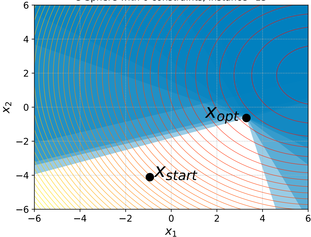
3 Sphere with 6 constraints, instance=13
