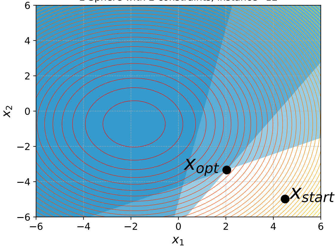
2 Sphere with 2 constraints, instance=12
