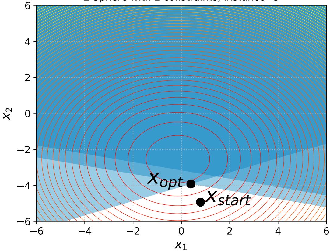
2 Sphere with 2 constraints, instance=5
