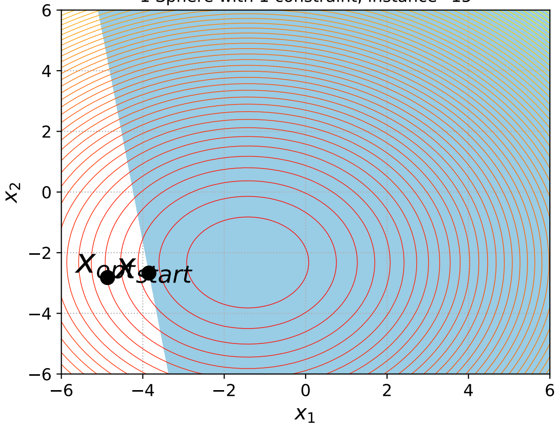
1 Sphere with 1 constraint, instance=15
