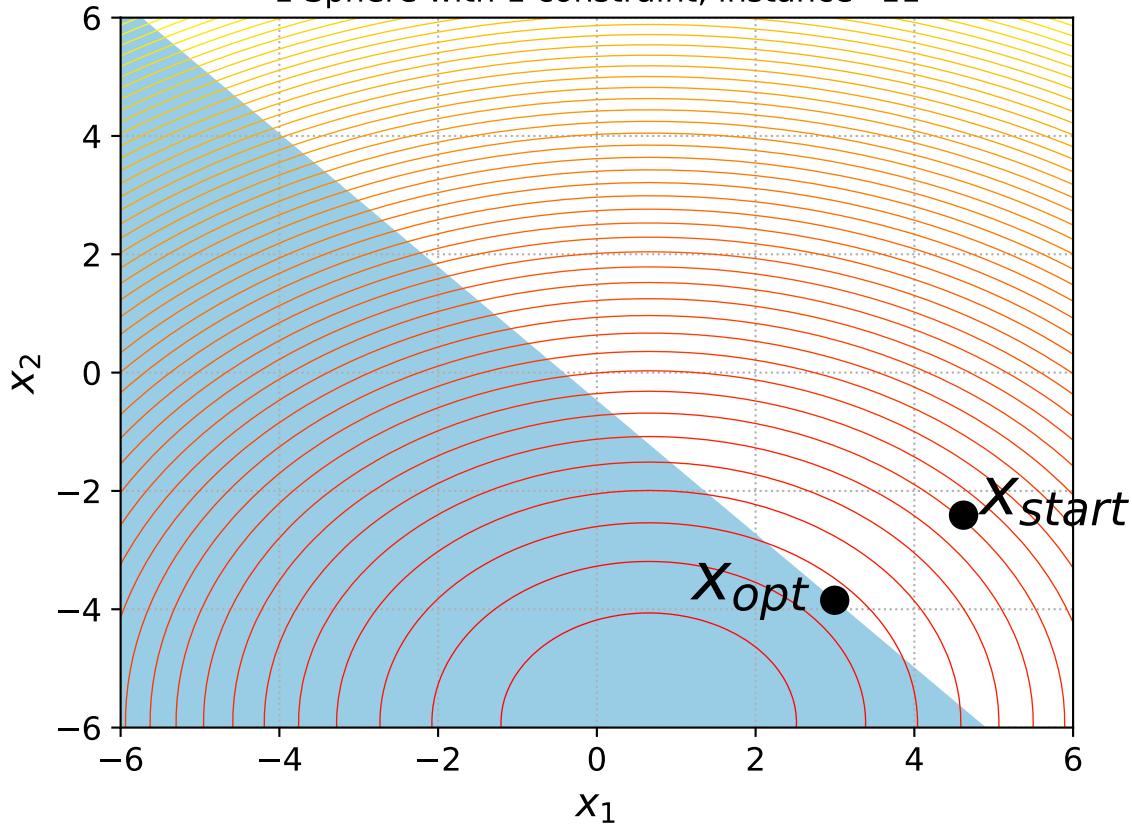
1 Sphere with 1 constraint, instance=11
