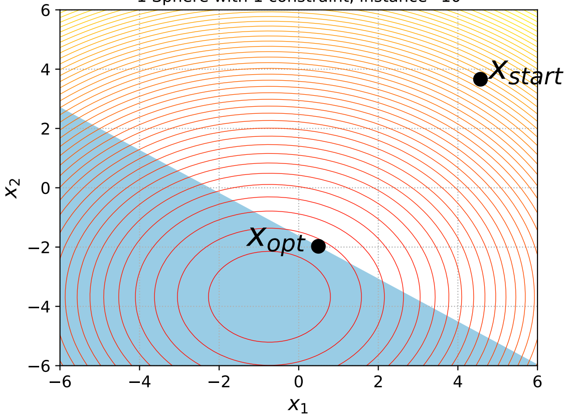
1 Sphere with 1 constraint, instance=10
