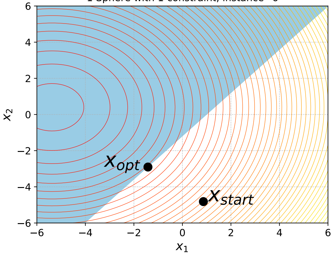
1 Sphere with 1 constraint, instance=6
