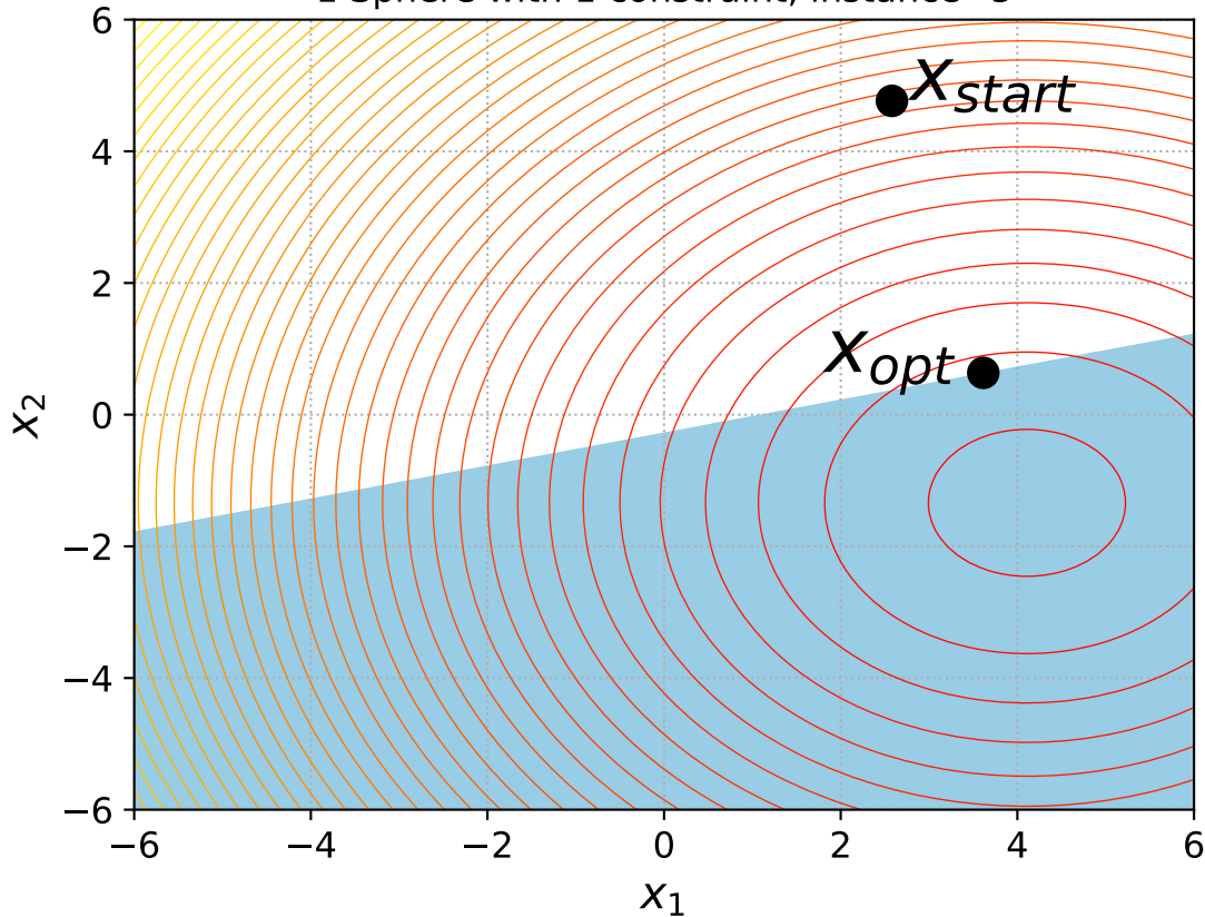
1 Sphere with 1 constraint, instance=5
