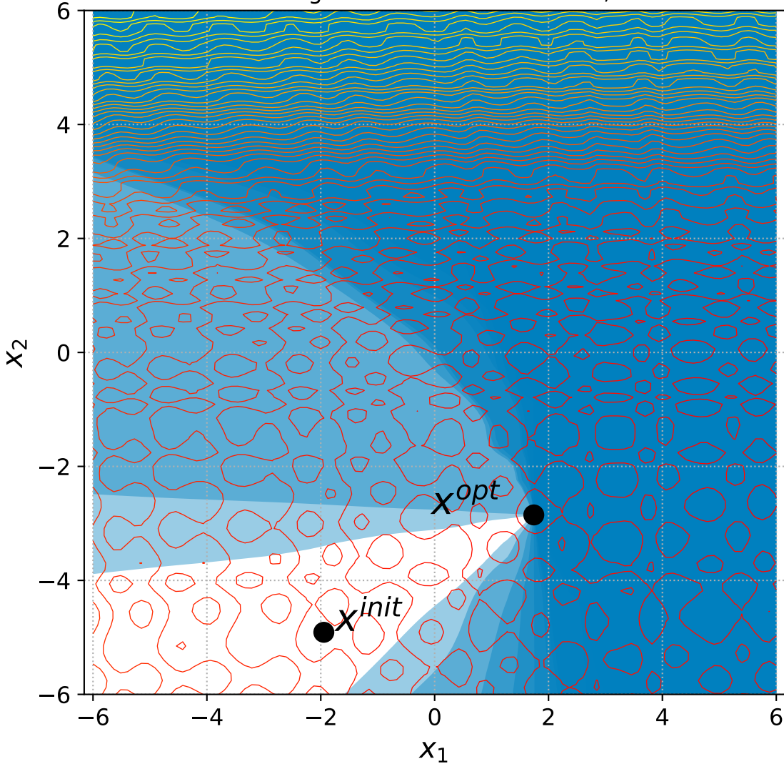
54 Rotated Rastrigin with 6+3n constraints, instance=15
