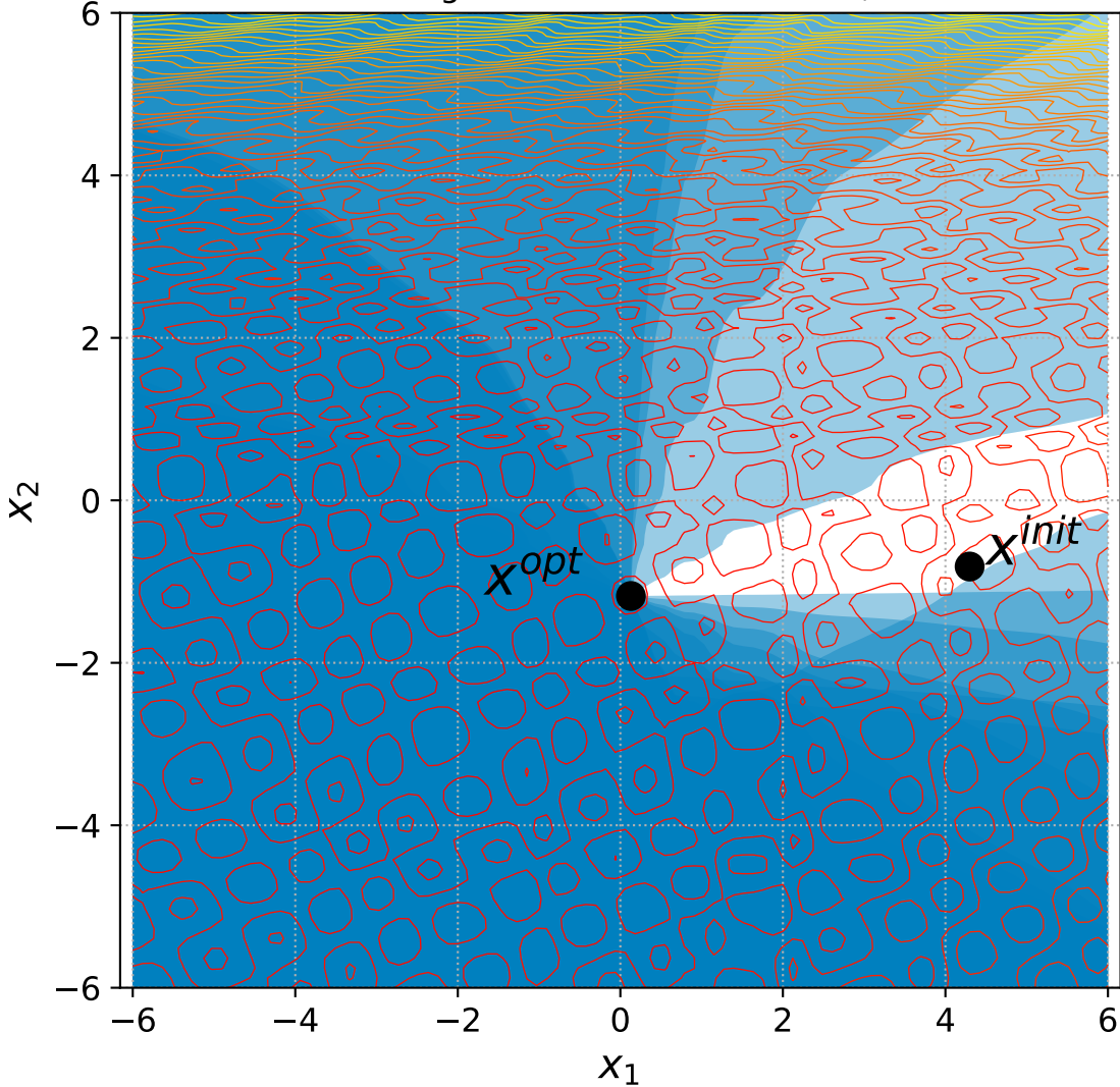
54 Rotated Rastrigin with 6+3n constraints, instance=14
