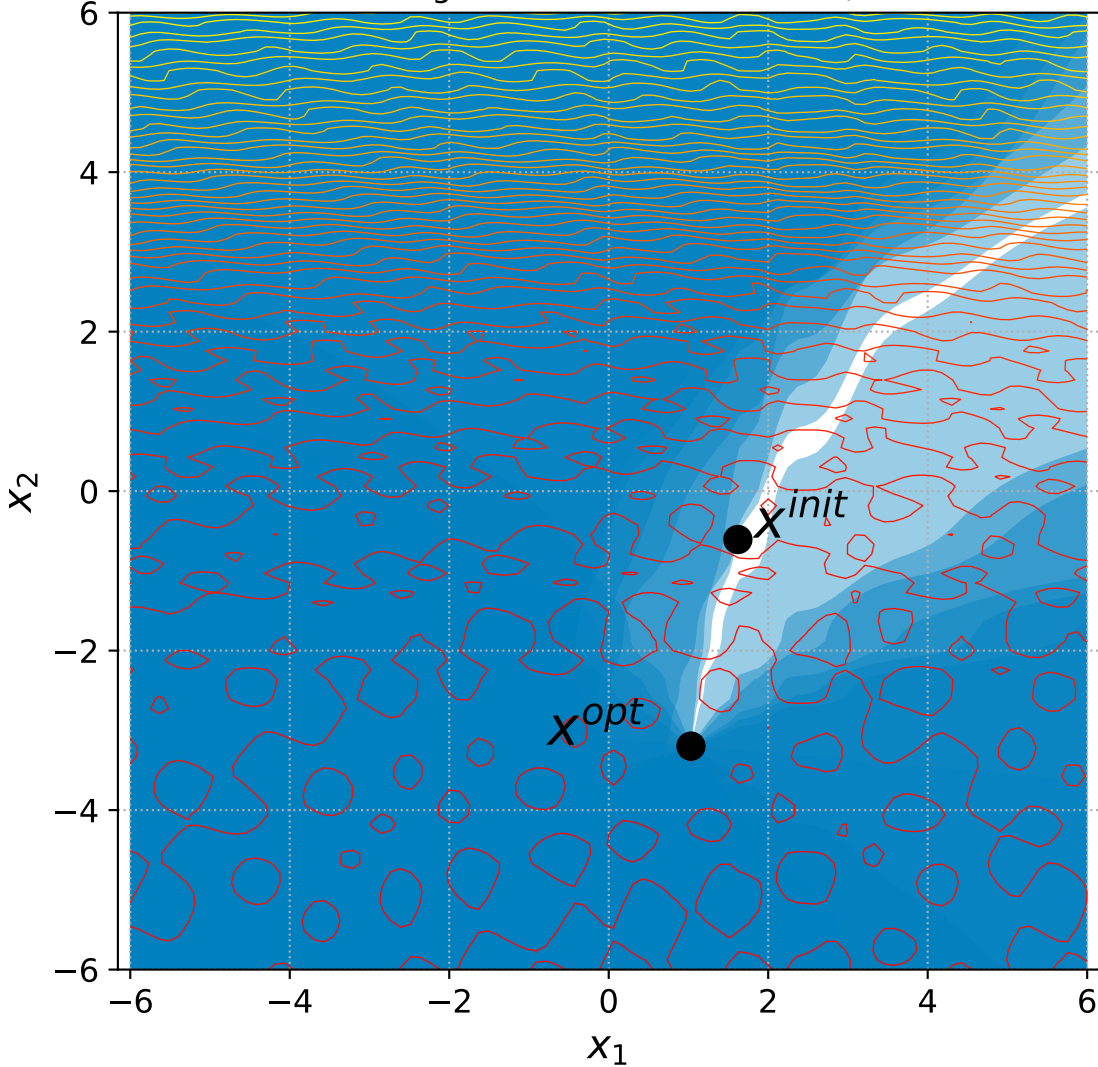
54 Rotated Rastrigin with 6+3n constraints, instance=13
