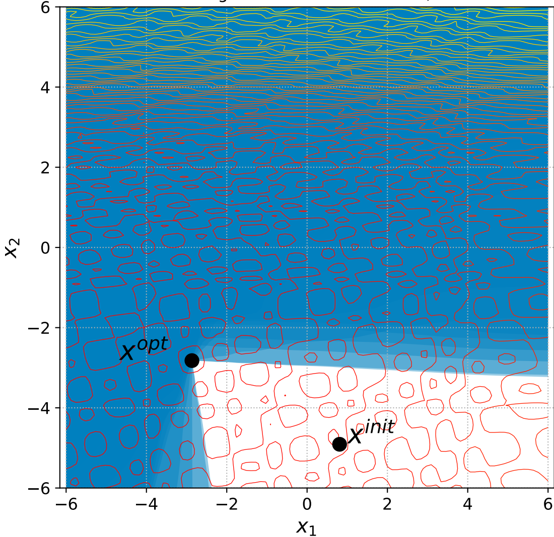
54 Rotated Rastrigin with 6+3n constraints, instance=10
